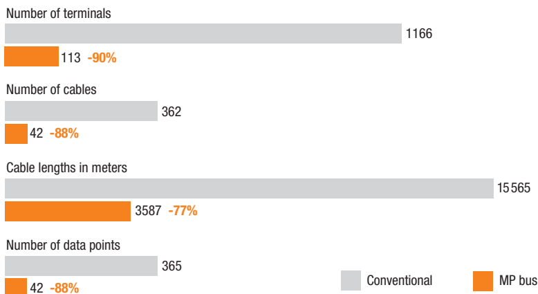
Massive savings in Sälipark Olten thanks to MP bus technology
